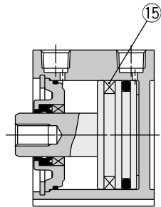
With auto switch magnet
