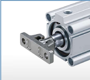
Simple joint A
