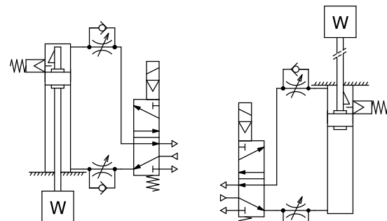
With head end lock
