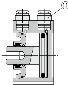
Built-in One-touch fittings
