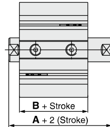
Double acting, Double rod/ Large bore
