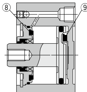
With rubber bumper
