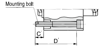
Non-rotating rod end mounting
