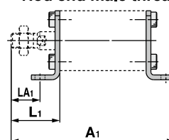
Rod end male thread
