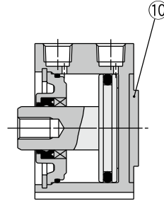
With boss on head end
