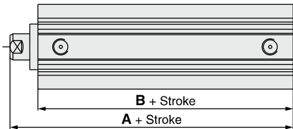
Double acting, Single rod/ Long stroke
