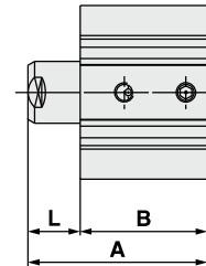
Single acting, Spring extend
