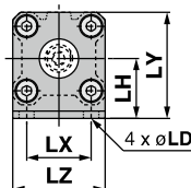
Without auto switch magnet CQ-LC0 □□
