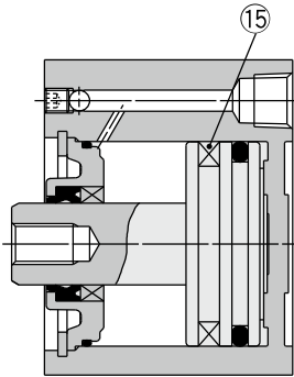
With auto switch magnet
