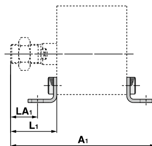
Rod end male thread
